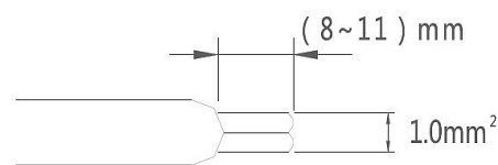
Figura 3-5-2 Conductor desnudo
