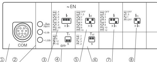
Diagram 9. NM8N-400, 630 EN 4C ( Power distribution ) Controller interface
